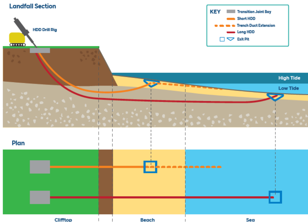
Plate 5-8 Illustrative Section and Plan Landfall Works HDD options
